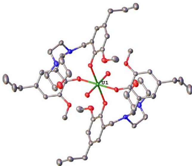
Figure 6. Thermal ellipsoid projection of [\text{UO}_2(\text{N}',\text{N}'\text{-bis}(2\text{-hydroxy-3-methoxy-5-(propen-2-yl)benzyl-N-(2-aminoethyl)-morpholine})_2]\cdot 2\text{CH}_3\text{CN} . The carbon atoms are depicted in gray, the oxygen atoms red, and the nitrogen atoms blue, the central uranium atom is in green, and the hydrogen atoms are omitted for clarity. 105,142
