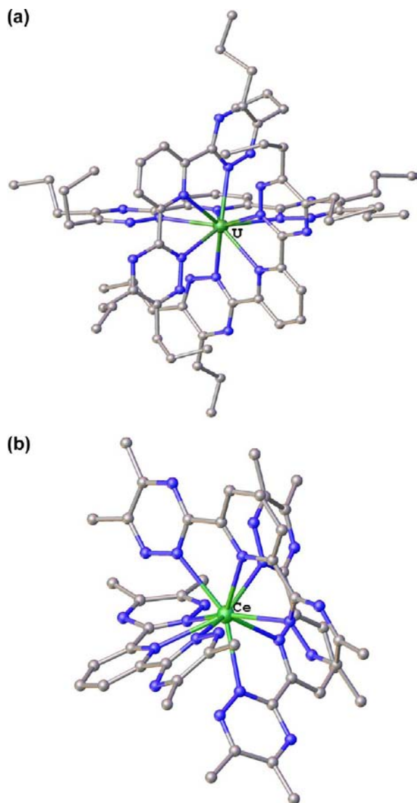
Figure 3. Projections of (a) [\text{U}(\text{Pr}^m \text{btp})_3]^{3+} and (b) [\text{Ce}(\text{Mebtp})_3]^{3+} . Ball-and-stick models are shown, lacking hydrogen atoms for clarity. The carbon atoms are depicted in gray, the oxygen atoms red, the nitrogen atoms blue, and the f element atoms green. 105,142
