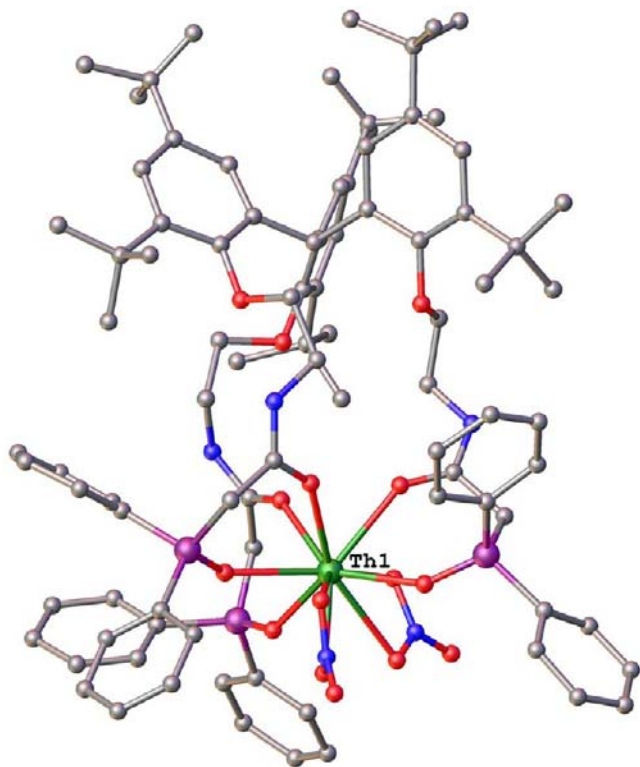
Figure 1. Projection of [\text{tris}(3,5\text{-tert-butyl-2-}((\text{diphenylphosphoryl})\text{-acetamido)ethoxy)phenyl})\text{Th}(\text{NO}_3)_2](\text{NO}_3)_2] . The carbon atoms are depicted as gray, the oxygen red, the nitrogen blue, and the central thorium atom green. For clarity, the structure is shown as a ball and stick projection and hydrogens have been omitted for clarity. 64,142
